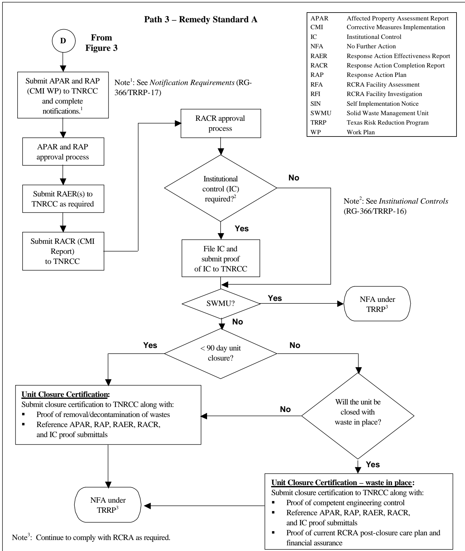
Figure 5. Path 3 – Remedy Standard A - TRRP Corrective Action Process
