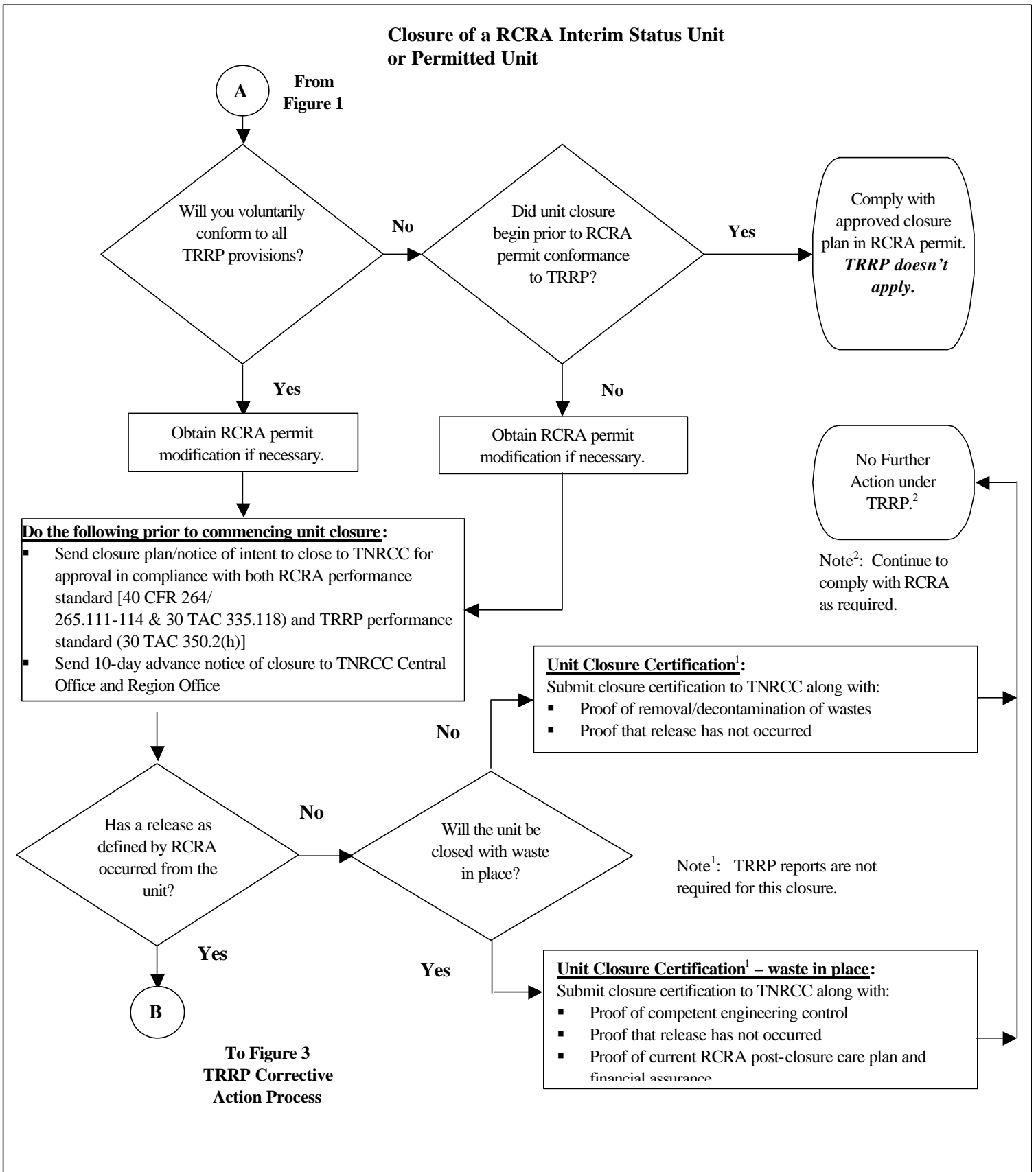
Figure 2. Closure of a RCRA Interim Status Unit or Permitted Unit
